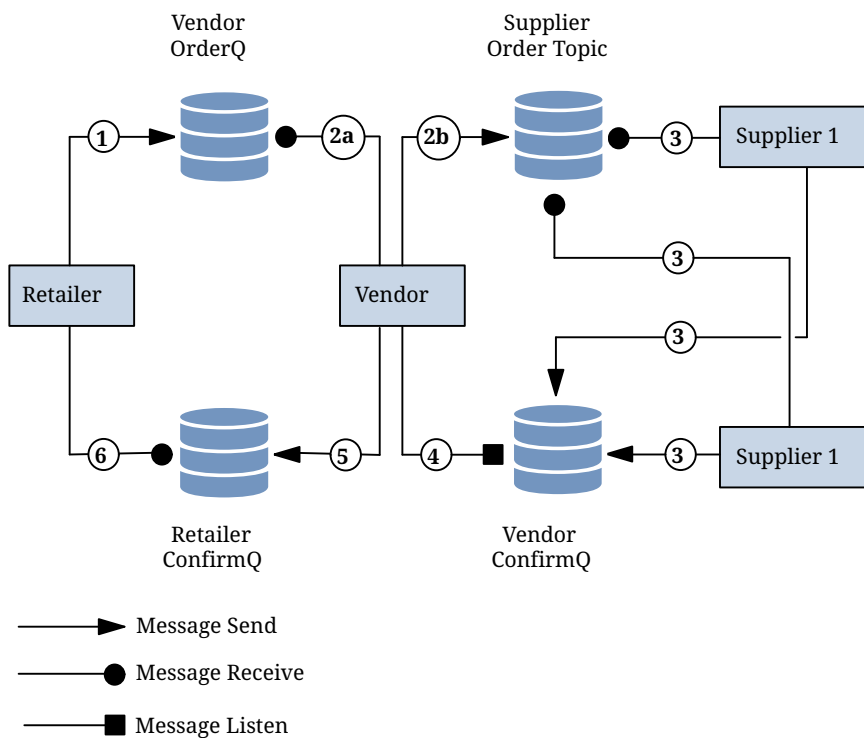
Figure 32. Transactions: Messaging Client Example
